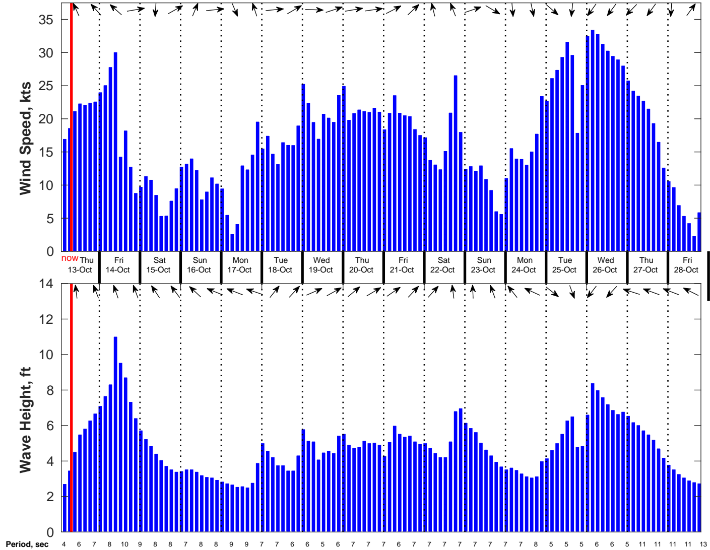
Wind & Wave Forecast for Vineyard Wind GB22 from 13-Oct-2022 02:00:00 to 29-Oct-2022 02:00:00
